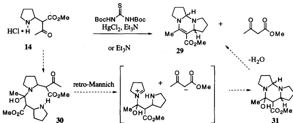
Scheme 4. Proposed Mechanism for the Formation of 29 .
