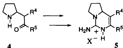
Scheme 2. Synthetic strategy
