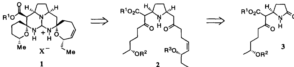
Scheme 1. Retrosynthetic analysis.
