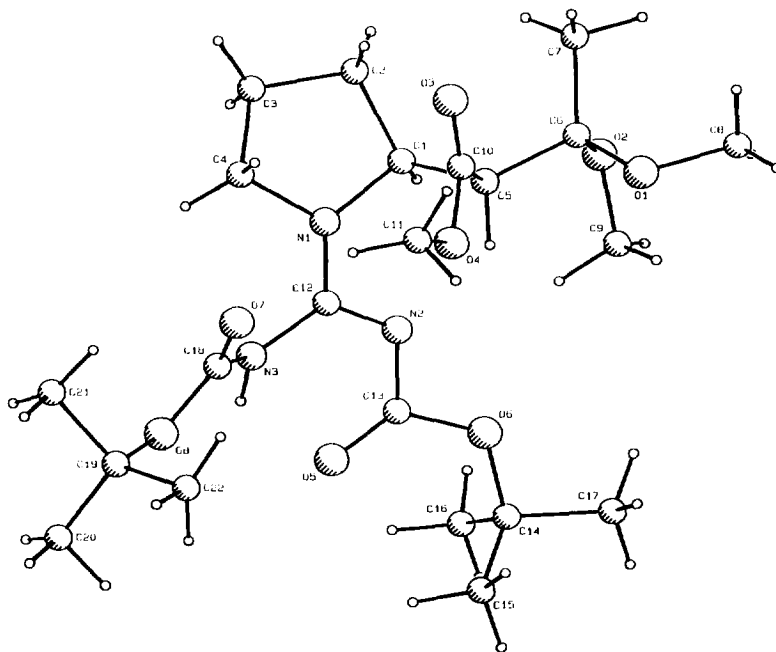
Figure 2. ORTEP-diagram of 39a .
