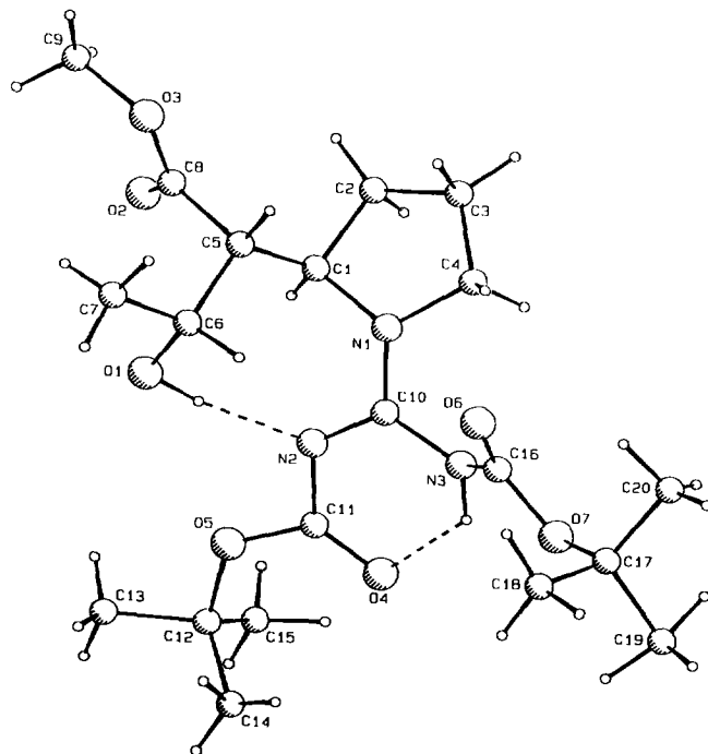
Figure 1. ORTEP-diagram of 34a .
