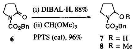
Scheme 3. Synthesis of the precursor
